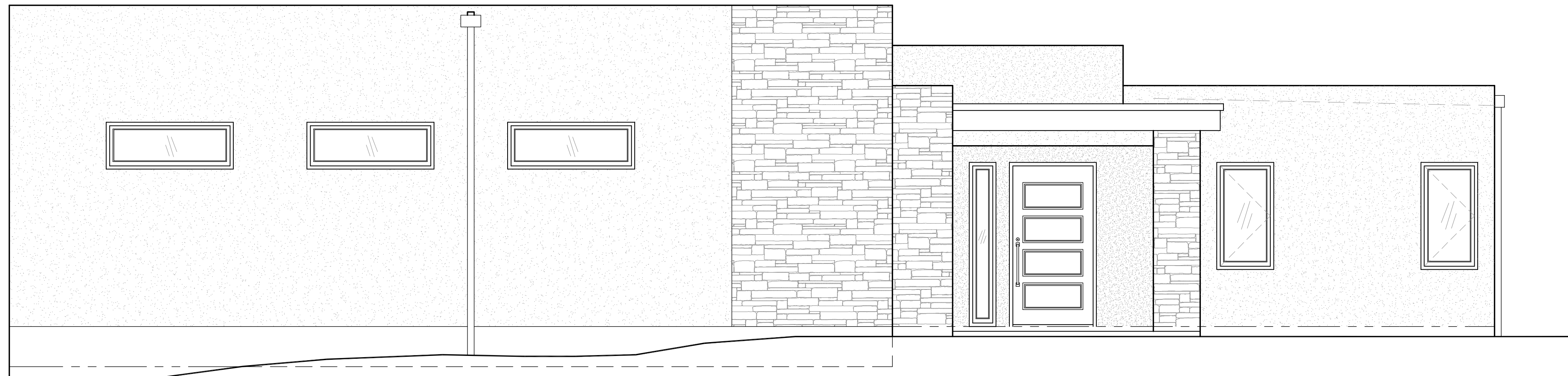
FRONT VIEW
