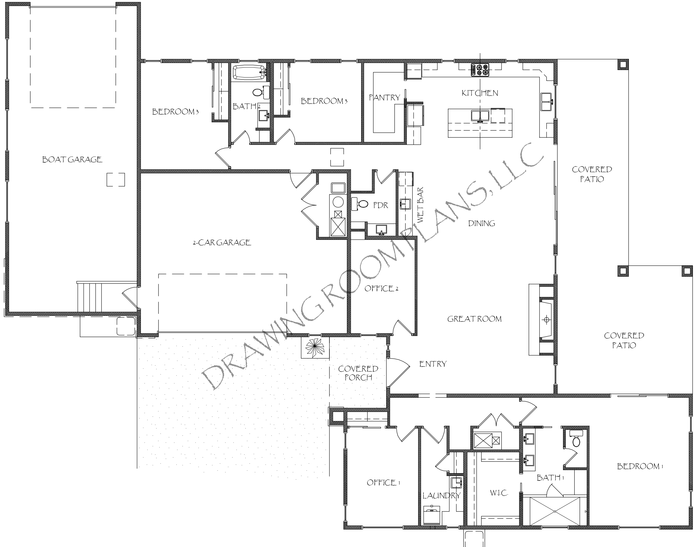
FLOOR PLAN
